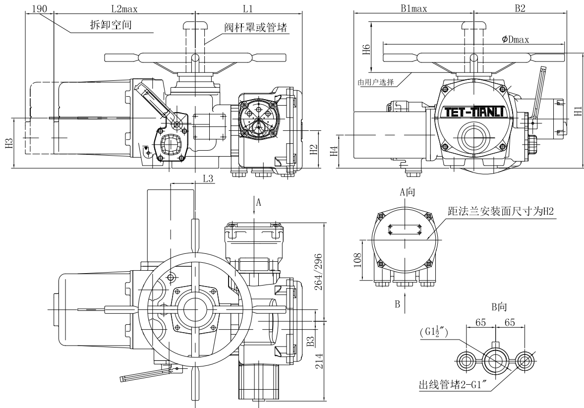
SMC-04~03防爆型、整体防爆型外形尺寸
